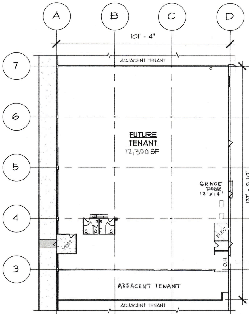
1 BLDG. 100 - SUITE 160 SCALE: 1/32" = 1'-0"
